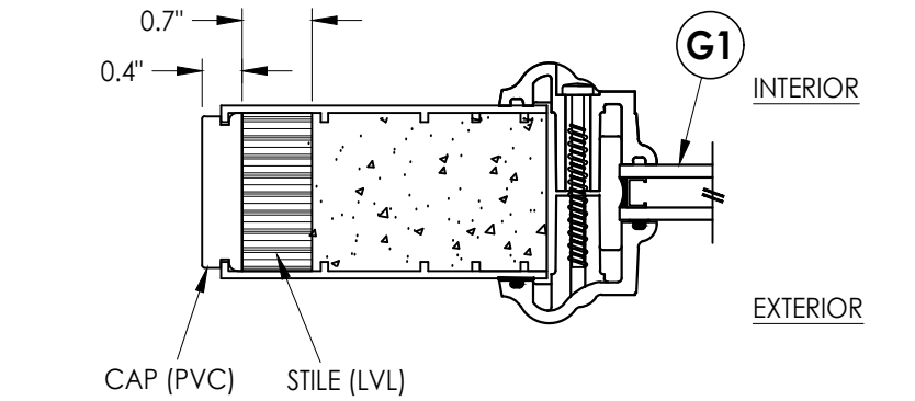
1 4 HORIZONTAL CROSS SECTION
