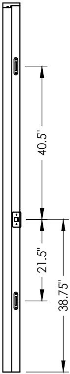
STRIKE MULLION Multi-point Lock (Vented Sidelite)
