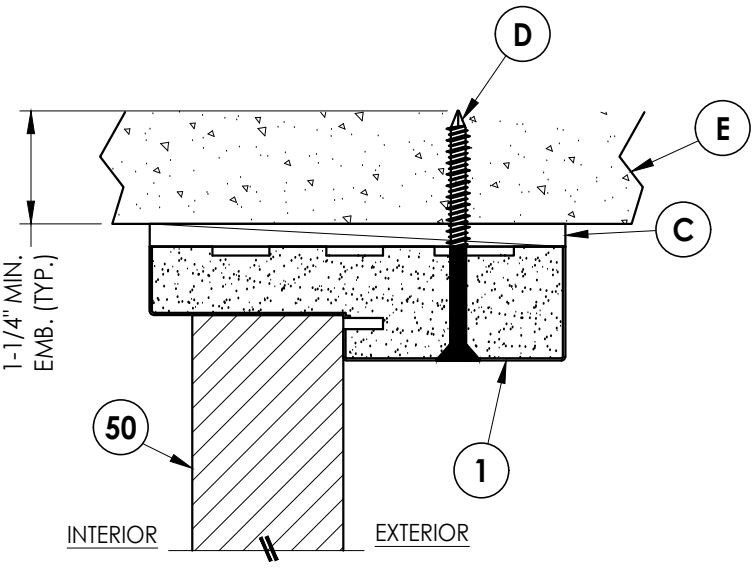
2 VERTICAL CROSS SECTION 8 Inswing shown Direct to Masonry Construction
