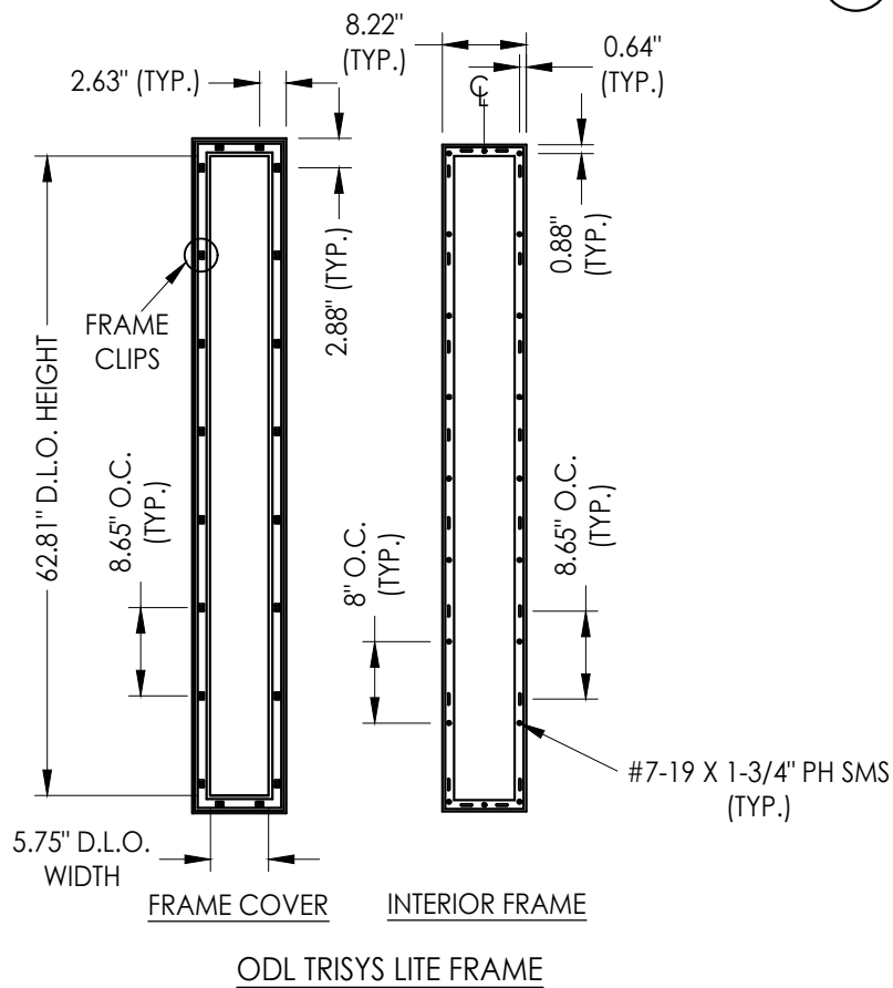
3A ODL LITE FRAME (TriSys) HP Polypropylene (Interior Frame) PC ABS (Exterior Frame, Frame Cover)
