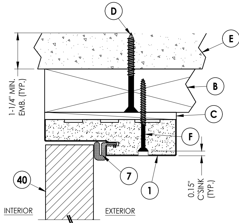
1 6 VERTICAL CROSS SECTION Inswing shown 2X Buck Construction
