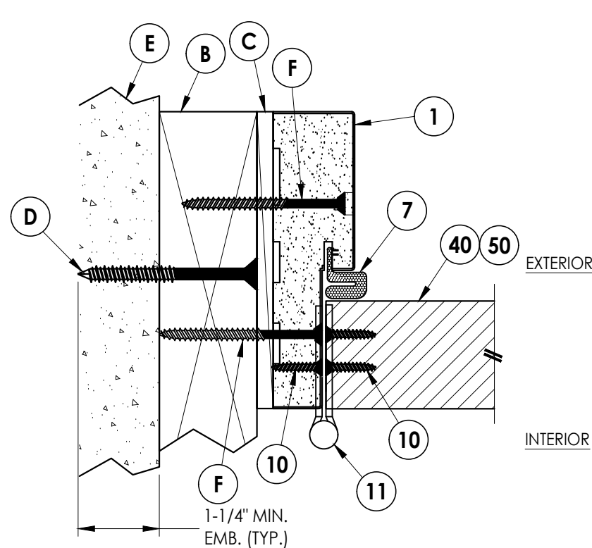
3 6 HORIZONTAL CROSS SECTION Inswing shown 2X Buck Construction
