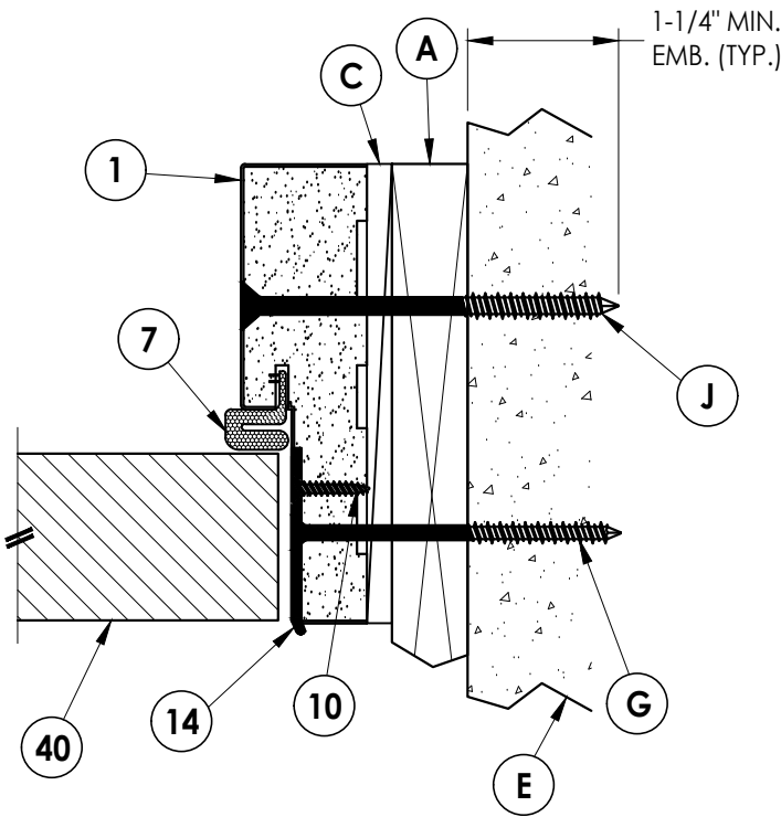
4 7 HORIZONTAL CROSS SECTION Inswing shown 1X Buck Construction
