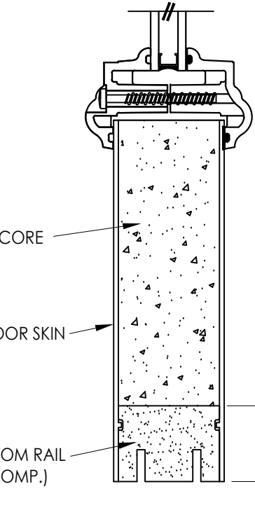
2 4 VERTICAL CROSS SECTION
