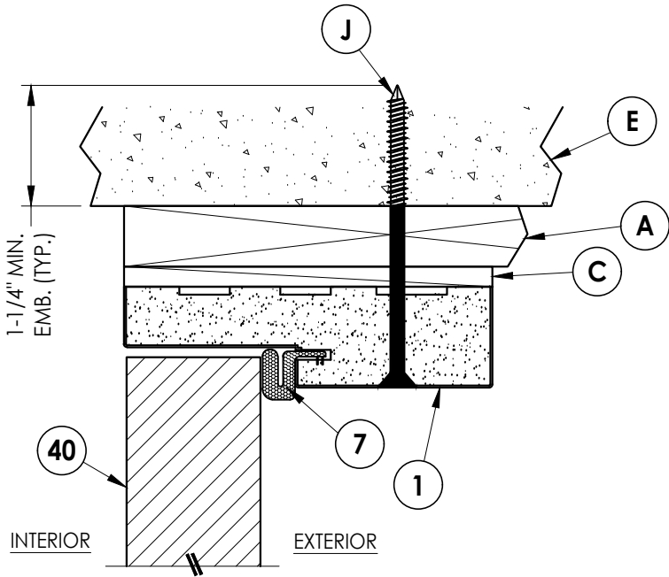
1 7 VERTICAL CROSS SECTION Inswing shown 1X Buck Construction
