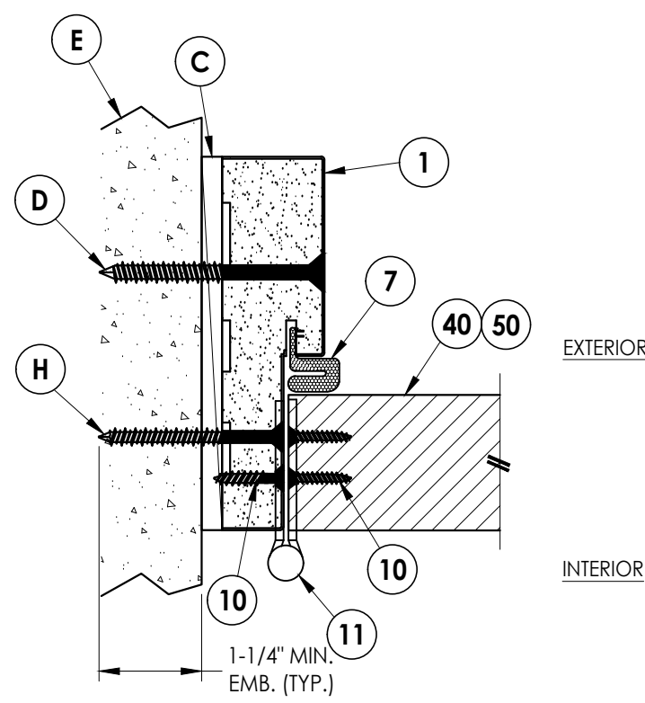
3 HORIZONTAL CROSS SECTION 8 Inswing shown Direct to Masonry Construction
