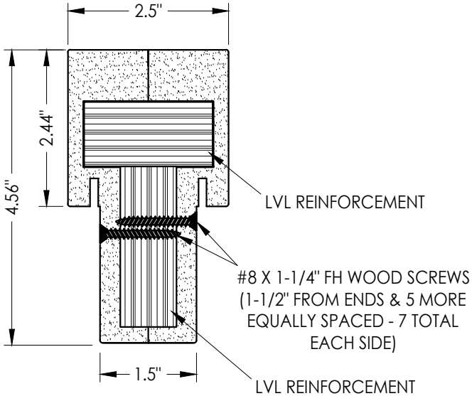
2 INTEGRAL MULLION
