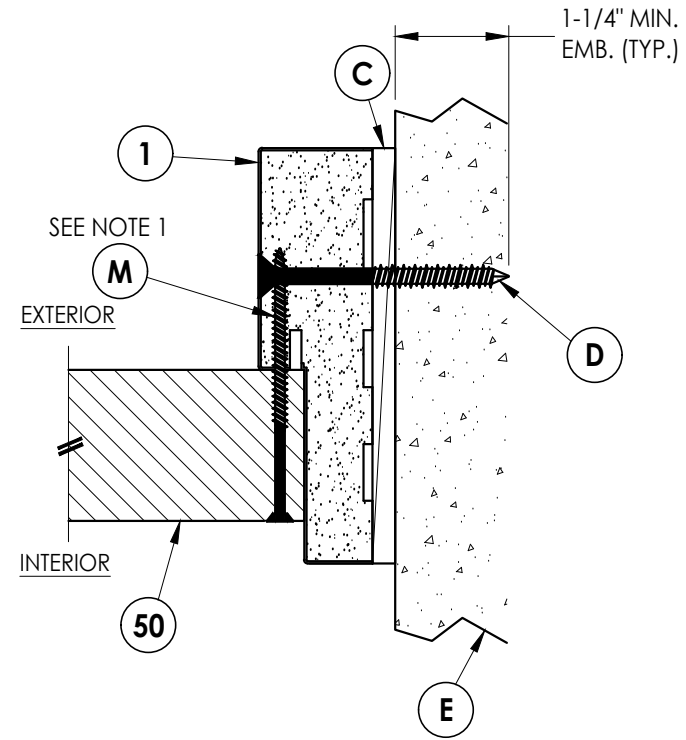
5 HORIZONTAL CROSS SECTION 8 Inswing shown Direct to Masonry Construction
