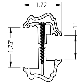
3A ODL LITE FRAME (TriSys) HP Polypropylene (Interior Frame) PC ABS (Exterior Frame, Frame Cover)
