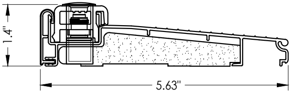
20 INSWING THRESHOLD Endura (Z-Series)
