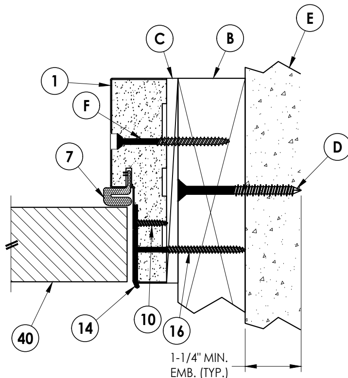
4 6 HORIZONTAL CROSS SECTION Inswing shown 2X Buck Construction
