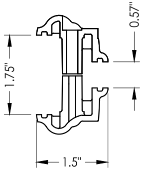
4A ODL LITE FRAME HP Polypropylene
