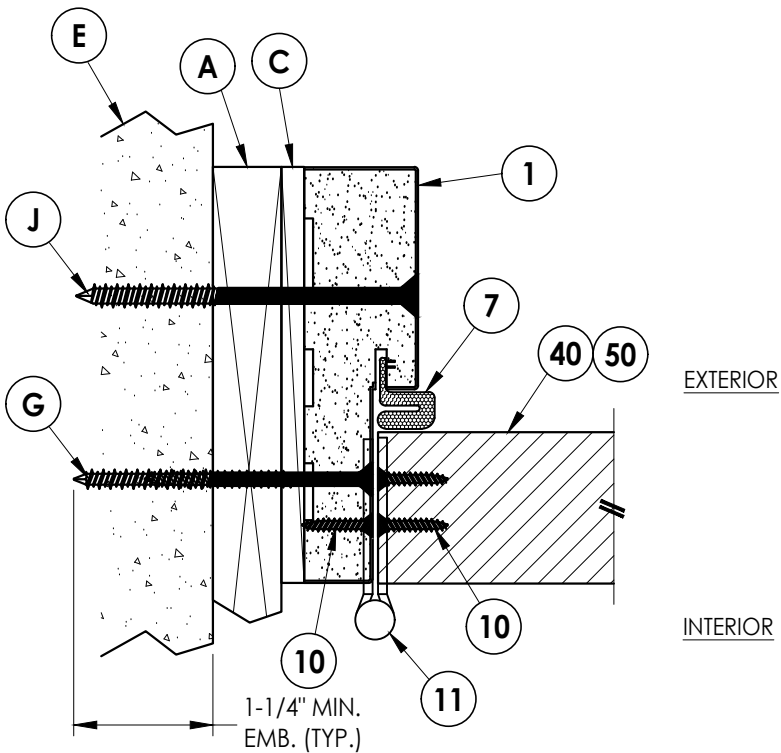
3 7 HORIZONTAL CROSS SECTION Inswing shown 1X Buck Construction
