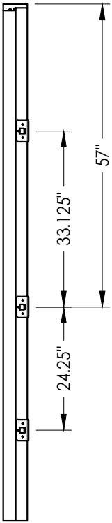
STRIKE JAMB/MULLION Multi-point Lock (Door)
