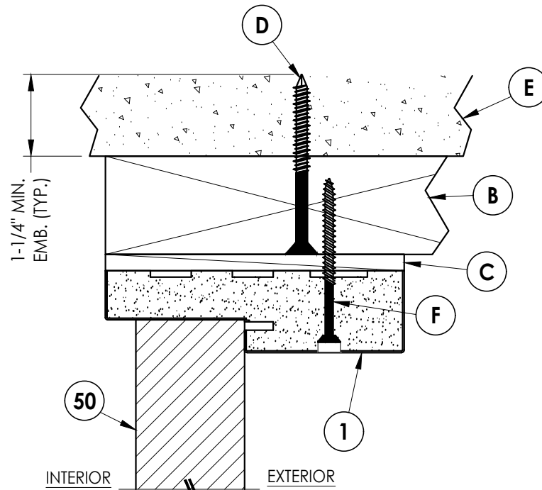
2 6 VERTICAL CROSS SECTION Inswing shown 2X Buck Construction
