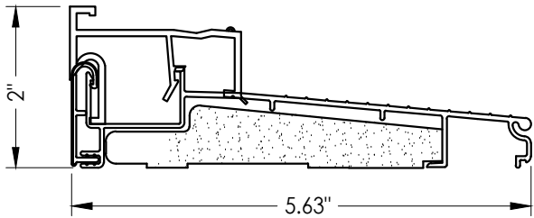
21 INSWING THRESHOLD w/ SIDELITE ADAPTER Endura (Z-Series)
