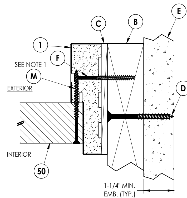
5 6 HORIZONTAL CROSS SECTION Inswing shown 2X Buck Construction
