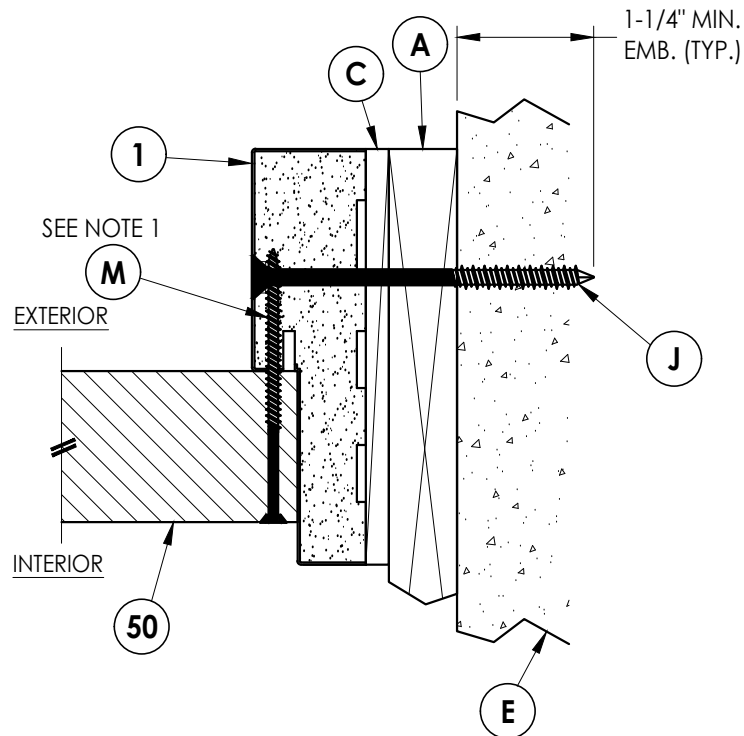
5 7 HORIZONTAL CROSS SECTION Inswing shown 1X Buck Construction
