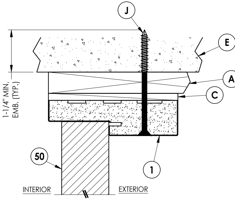
2 7 VERTICAL CROSS SECTION Inswing shown 1X Buck Construction
